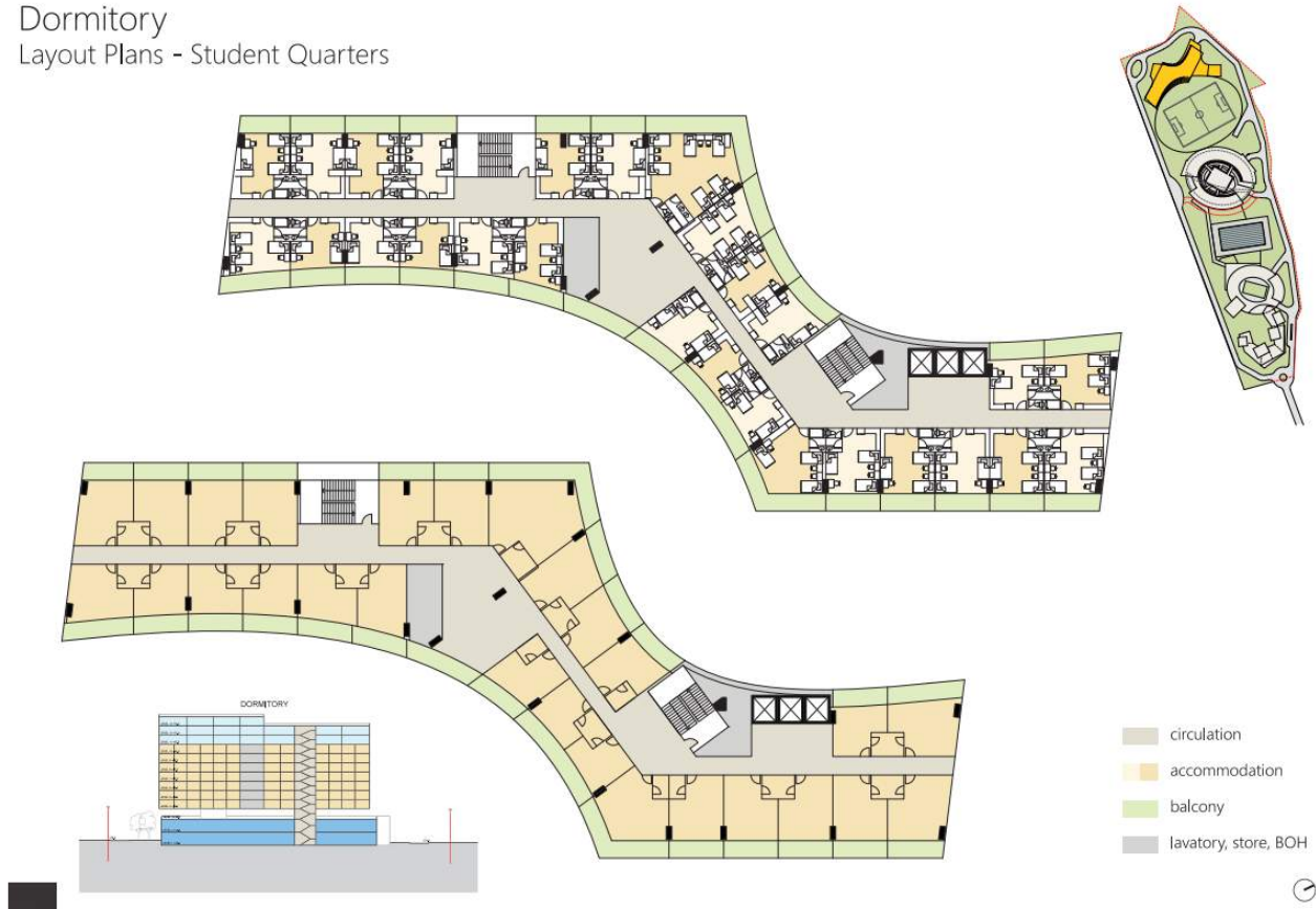
Dragon House layout plans
